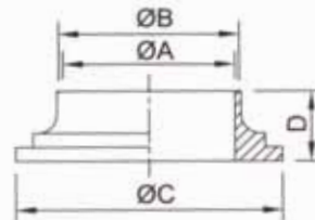
Long Welding Liner SMS-14
