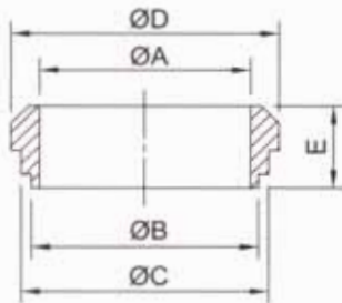
3A Short Bevel Seat Weld Liner 3A-14PRF
