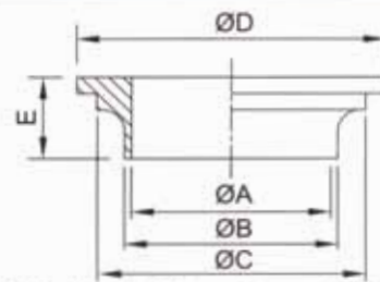
CL-Style Welding Liner SMS-14G
