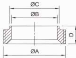
3A Short Bevel Seat Weld Male 3A-15TRF
