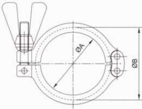
13CS DOUBLE PIN CLAMP
