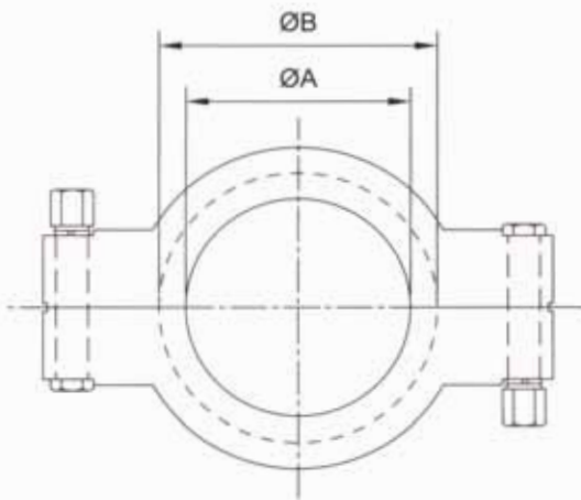
13MHP HIGH PRESSURE CLAMP WITH SCREW BOLT BRASS NUT
