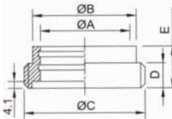
SMS Expanding Male 15R
